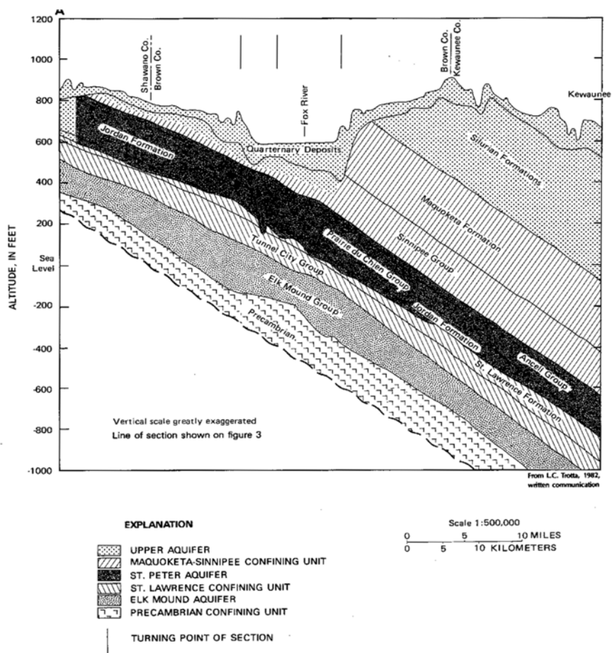
Figure 5. Diagram of hydrogeologic and stratigraphic units in the Lower Fox River Basin.
