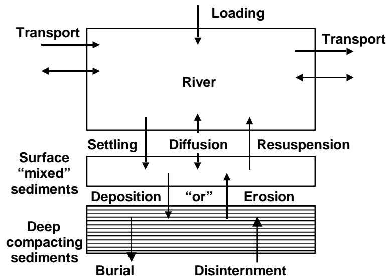
Figure 6. Schematic representation of major mechanisms governing transport and fate of solids in the Lower Fox River.
